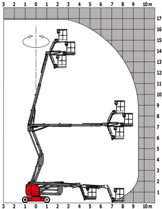
Laaddiagram
